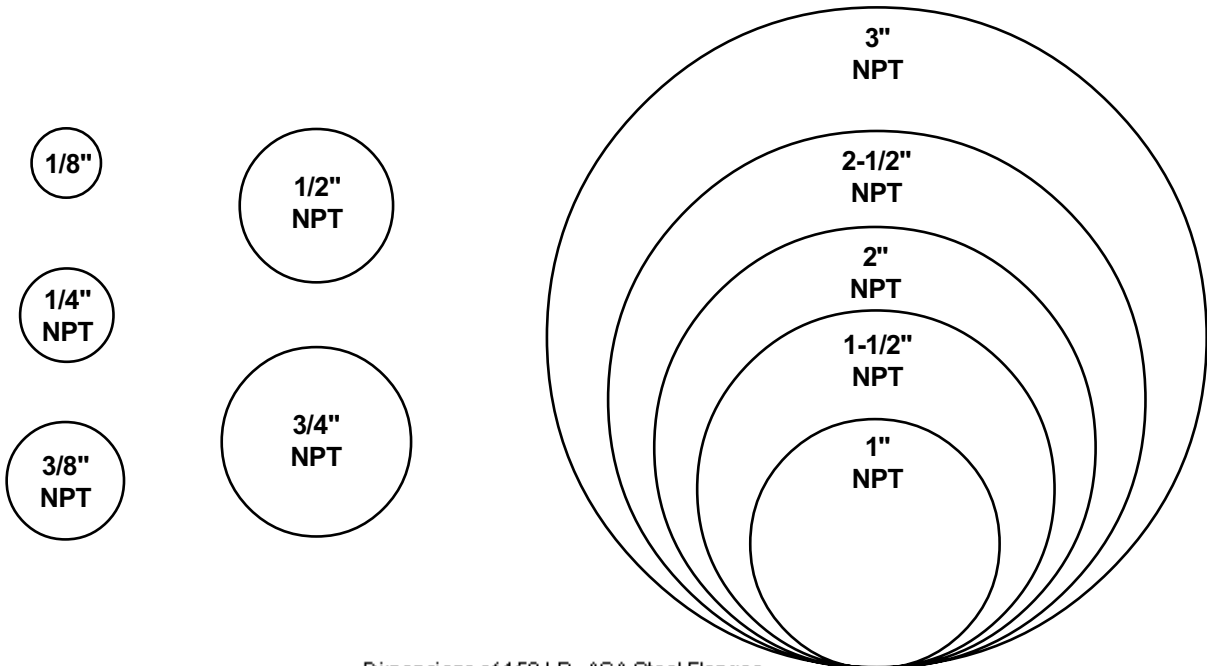
Dimensions of 150 LB. ASA Steel Flanges
